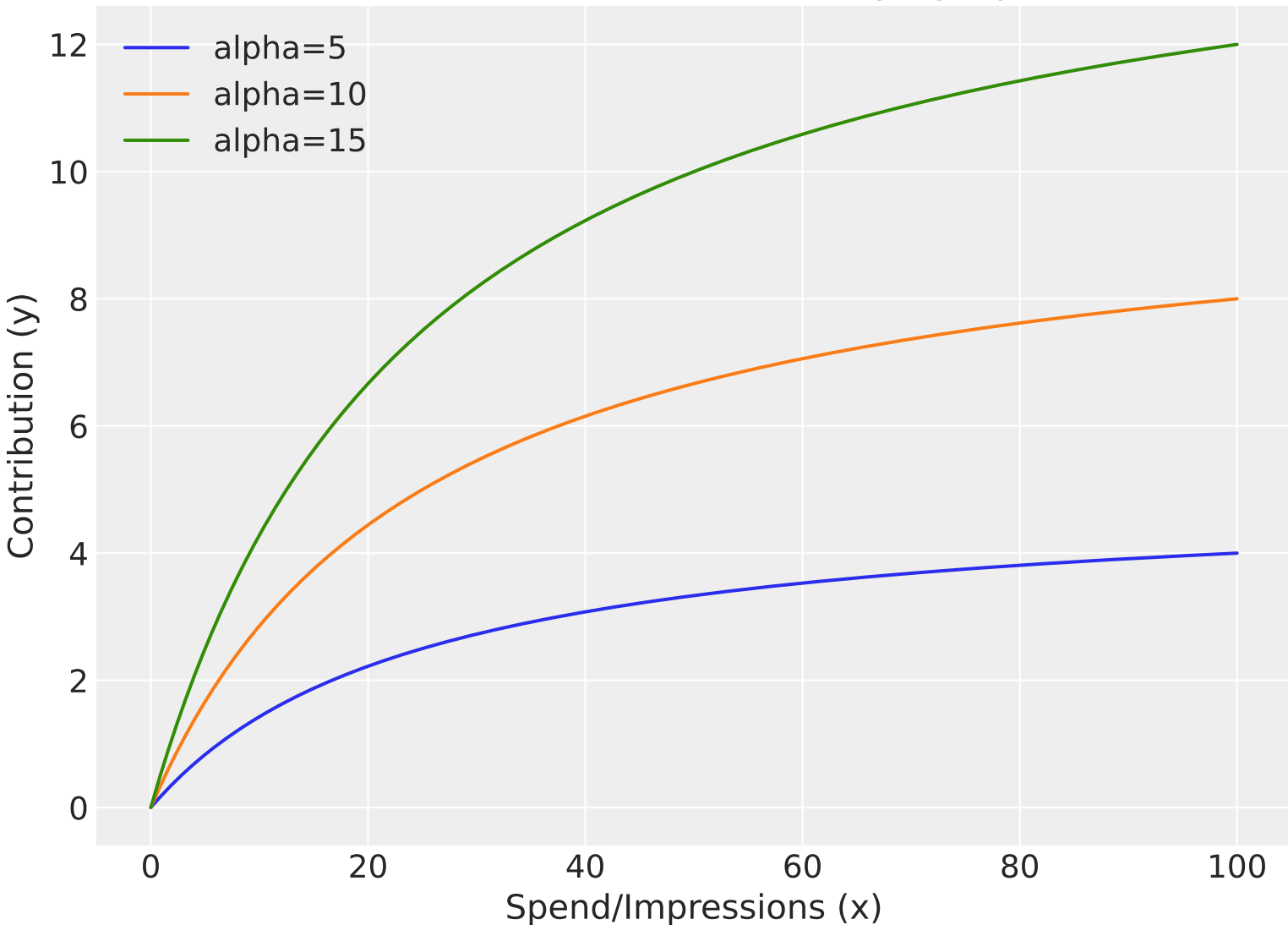
Michaelis-Menten Function (Varying alpha)
